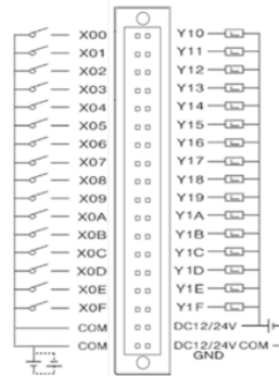
CM3-SP32PDTF 입력-출력
